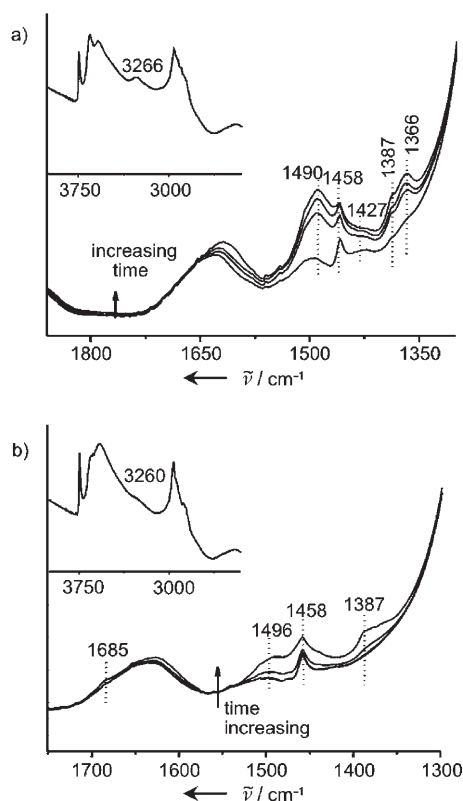
Figure 1. Time-resolved FTIR spectra of a) H-Mordenite at 6, 17, 23, and 49 min and b) Cu-H-Mordenite at 1, 5, 15, and 40 min, after CO/MeOH co-adsorption at 240°C. The insets show the 4000–2500 cm −1 IR region.
